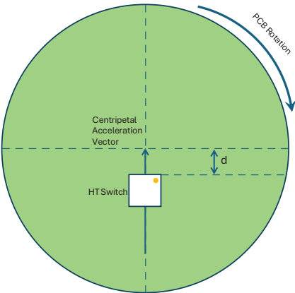
This diagram provides guidance on how to mount the switch for setback or impact detection.
