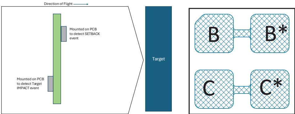
This diagram provides guidance on how to mount the switch for setback or impact detection.
