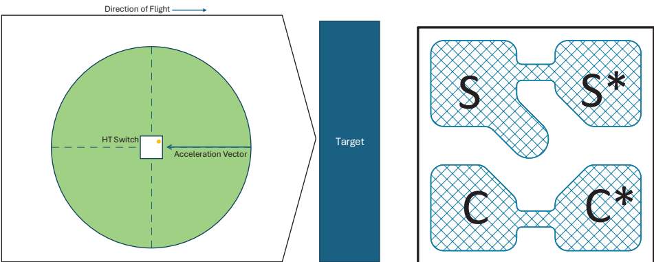
This diagram provides guidance on how to mount the switch for setback or impact detection.
