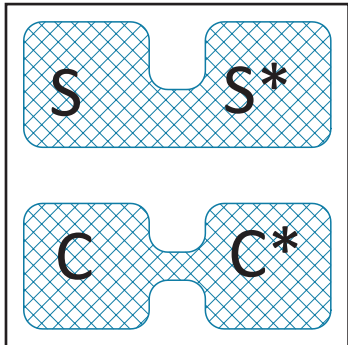
AT-12000-S7 Pad View
