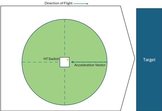
This diagram provides guidance on how to mount the switch for setback or impact detection.
