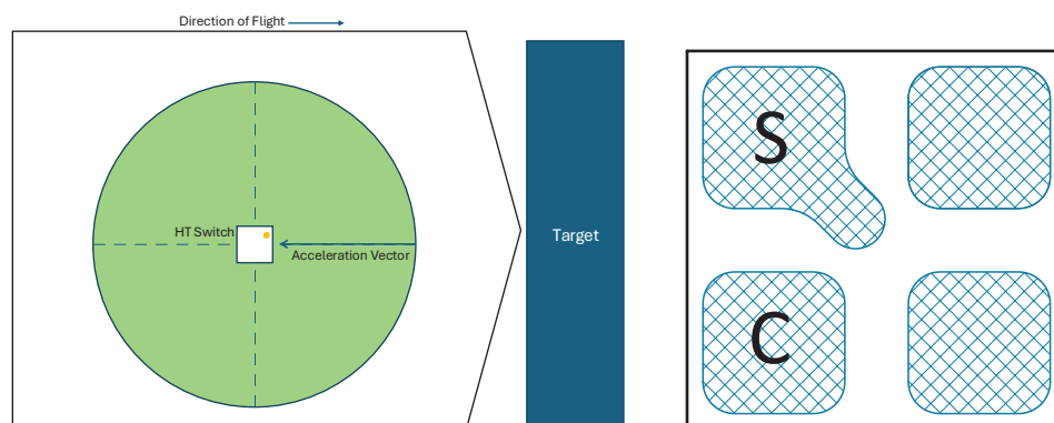
AT-25-S Pad View
