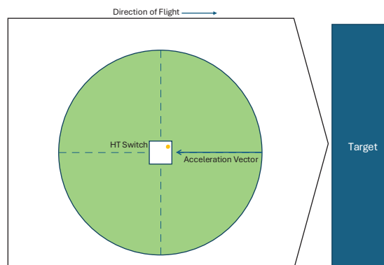
This diagram provides guidance on how to mount the switch for setback or impact detection.
