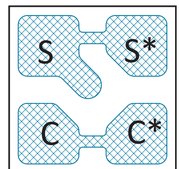
AT-12000-S Pad View
