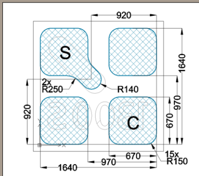
AT-1300-S Pad Dimensions (micrometers) as viewed from pad side of device
