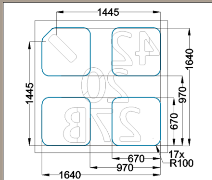
AT-27-B Pad Dimensions (micrometers) as viewed from pad side of device
